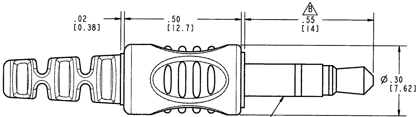
3.5MM STEREO PIN ASSEMBLY
